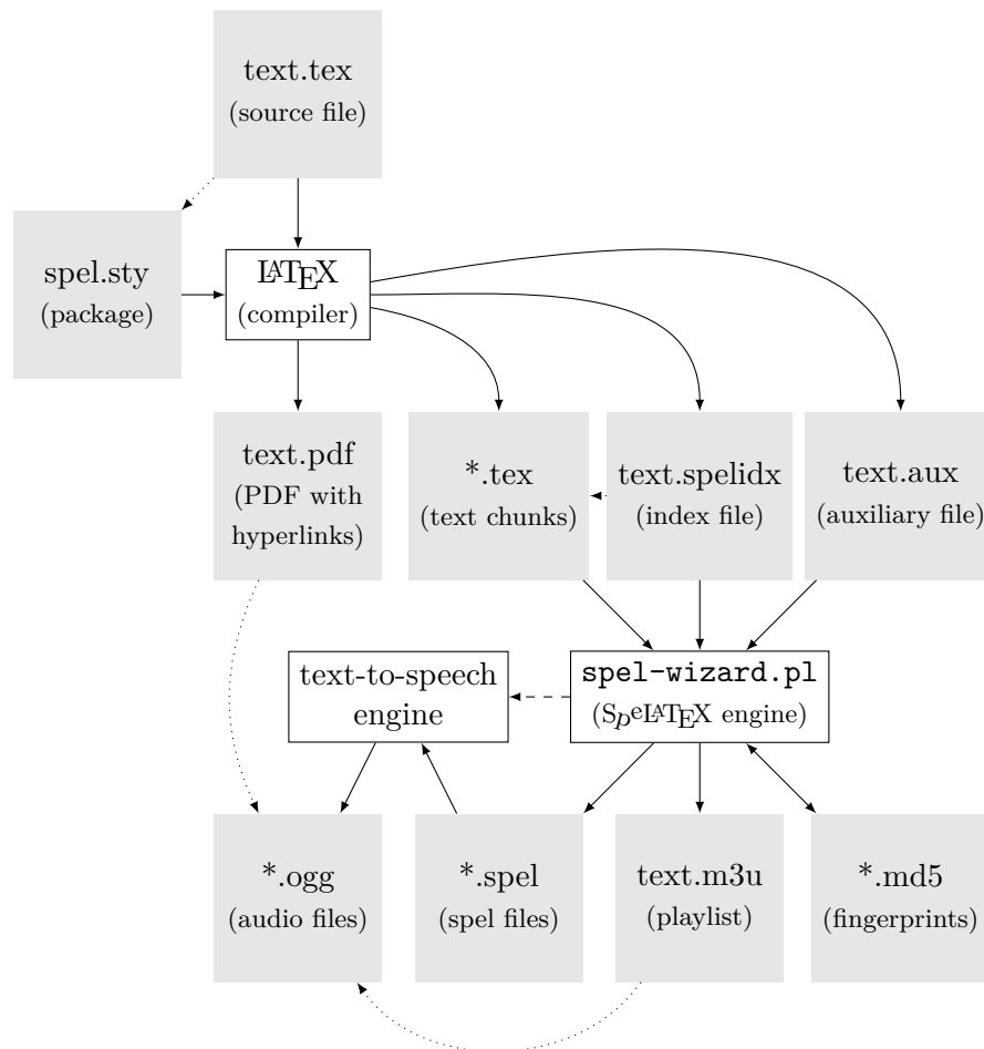
Figure 1: Basic tool setup of the S_{p^e}L_{A^T}E_X package; filled boxes indicate files, outlined boxes indicate tools; solid lines indicates use or creation of files, dotted lines indicate references, dashed lines indicate a control relationship.
